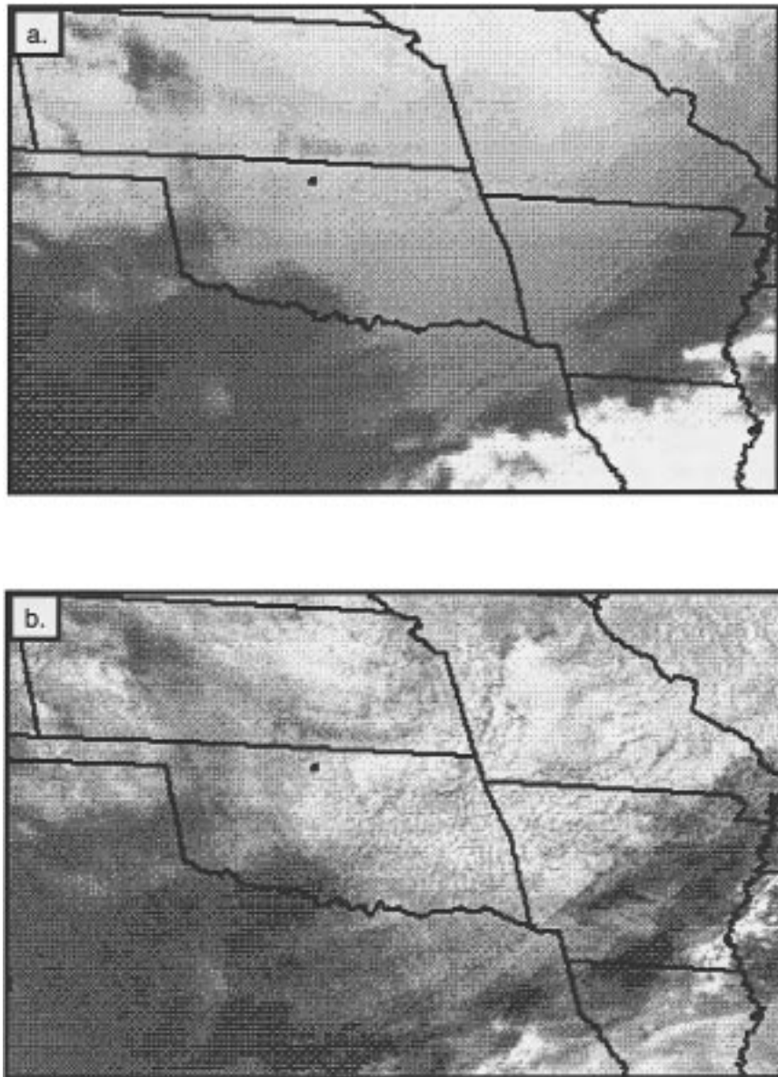
FIG. 1. Central United States (a) infrared 10-km and (b) visible 1-km resolution satellite images showing the extent of the stratus cloud outbreak at 2100 UTC on 30 April 1994.
