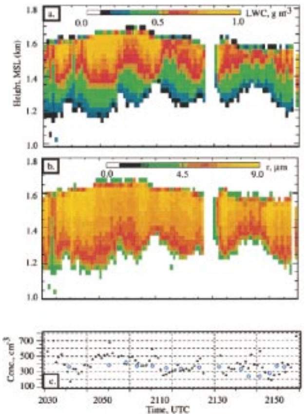
FIG. 8. Comparison of 1-min resolution (a) stratus LWC field using the variable N_d radar algorithm method, (b) radar-derived \bar{r} , and (c) a plot of radar-derived (*) and in situ ramp-averaged (O) N_d .
