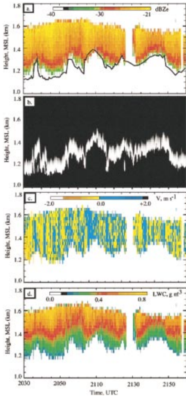
FIG. 6. High-resolution time-height displays of (a) K_a -band radar reflectivity factor Z_e (with lidar cloud-base heights shown by the line), (b) 0.532\text{-}\mu\text{m} lidar relative returned energy, (c) mean Doppler radar velocity V_r , and (d) radar algorithm-derived LWC using N_d = 347\text{ cm}^{-3} .
