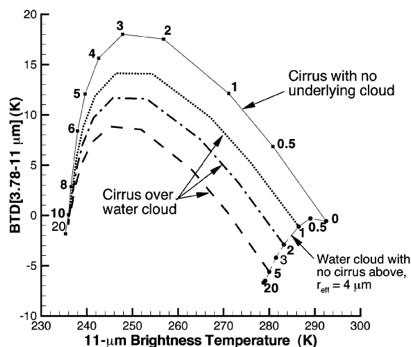
FIG. 5. Simulation of overlapping clouds (cirrus uncinus overlying a low-level water cloud) on brightness temperature differences as a function of 11\text{-}\mu\text{m} brightness temperature. The cirrus uncinus and water cloud temperatures are 235 and 285 K, respectively. Infrared cloud-layer optical thickness values ( \tau_{\text{IR}} ) are provided on the uppermost cirrus curve and the water-cloud curve for reference.
