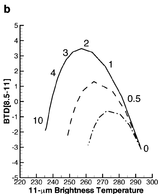
FIG. 4. Dependence of cloud temperature on brightness temperature differences as a function of 11\text{-}\mu\text{m} brightness temperature for ice-phase clouds at temperatures of 235, 248, and 261 K. Calculations are performed for (a) \text{BTD}(3.78\text{--}11) vs 11\text{-}\mu\text{m} brightness temperature and (b) \text{BTD}(8.5\text{--}11) vs 11\text{-}\mu\text{m} brightness temperature. The simulations were performed using the cold cirrus-scattering model and a midlatitude summer atmosphere. Infrared cloud layer optical thickness values ( \tau_{\text{IR}} ) are provided on the uppermost curve for reference.
