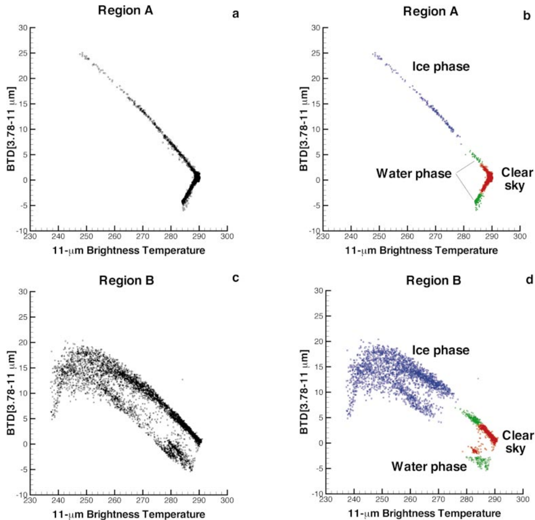
FIG. 8. Radiometric MODIS data from regions A and B are shown. (a) For region A, the \text{BT}_D(3.78\text{--}11\text{ }\mu\text{m}) is shown as a function of the 11\text{-}\mu\text{m} brightness temperature for the case of two nonoverlapping (i.e., single layered) clouds. (b) The MODIS operational products are used to identify the clear-sky pixels (red), the ice-phase cloud (blue), and the water-phase cloud (green). (c) For region B, the \text{BT}_D(3.78\text{--}11\text{ }\mu\text{m}) is shown as a function of the 11\text{-}\mu\text{m} brightness temperature for a more complex case containing both single-layered and multilayered clouds. (d) the MODIS operational products are used to identify the clear-sky pixels (red), the ice-phase cloud (blue), and the water-phase cloud (green).
