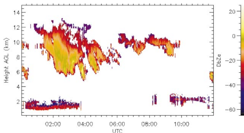
FIG. 10. Height-time cross section of radar reflectivity factor ( \text{dBZ}_e ) observed by the MMCR from 0000 to 1200 UTC 22 Apr 2001.
