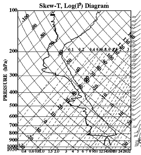
FIG. 7. Skew T -log p diagram from the sounding launched at 0535 UTC 22 Apr 2001. Pressure is denoted along the ordinate (hPa) while temperature ( ^\circ\text{C} ) extends diagonally from the lower left-hand to the upper right-hand side. The curved solid lines that run from the upper right-hand to lower left-hand side are the water saturation mixing ratio ( \text{g kg}^{-1} ), while mixing ratio lines ( \text{g kg}^{-1} ) are dashed. Wind barbs are shown with short tick marks denoting 5 \text{ m s}^{-1} and long ticks denoting 10 \text{ m s}^{-1} .
