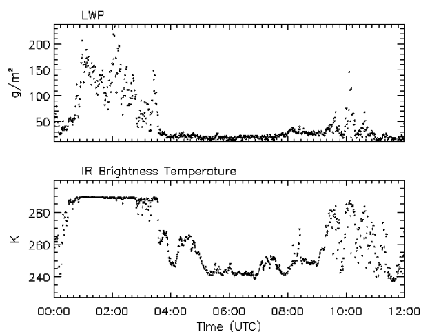
FIG. 11. (a) Liquid water path ( \text{LWP} , \text{g m}^{-2} ) derived from brightness temperatures observed by the microwave radiometer at the ARM Southern Great Plains site on 22 Apr 2001. The small residual value near zero after 0400 UTC can be considered zero LWP in this case. (b) IR brightness temperatures calculated from radiances observed by a narrow-field-of-view IR radiometer sensitive to radiation in the 9–11- \mu\text{m} region of the atmospheric window.
