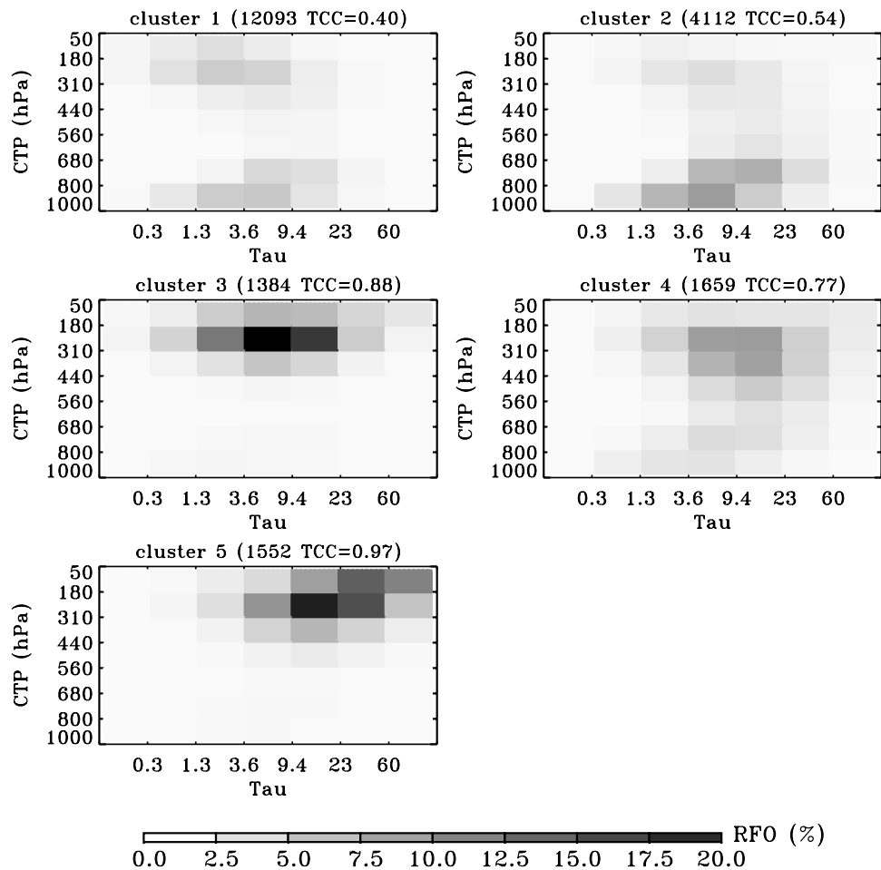
Figure 2. The cloud top pressure (CTP) – optical thickness (Tau) frequency histogram patterns from contemporary MODIS observations composited into the clusters from CloudSat data. The first number in brackets is the case number, and TCC is the MODIS total cloud cover and the integral over the entire histogram.
