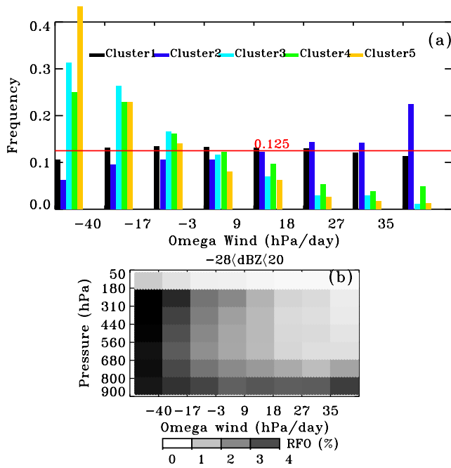
Figure 4. (a) The frequency of the occurrence for each cluster from CloudSat data as a function of the monthly mean vertical pressure velocity (Omega Wind) at 500 hPa calculated from NCEP analysis data. Each bin of the vertical velocity represents the equivalent occurrence frequency for the applied 500 hPa vertical pressure velocity. If there were no association of cluster regime with 500 hPa vertical pressure velocity, the frequency of occurrence for a given cluster would be 0.125 (red line) apart from random fluctuations. (b) The relative frequency of occurrence for valid dBZ range at a given pressure level as a function on the abscissa of the monthly mean 500 hPa vertical pressure velocity.
