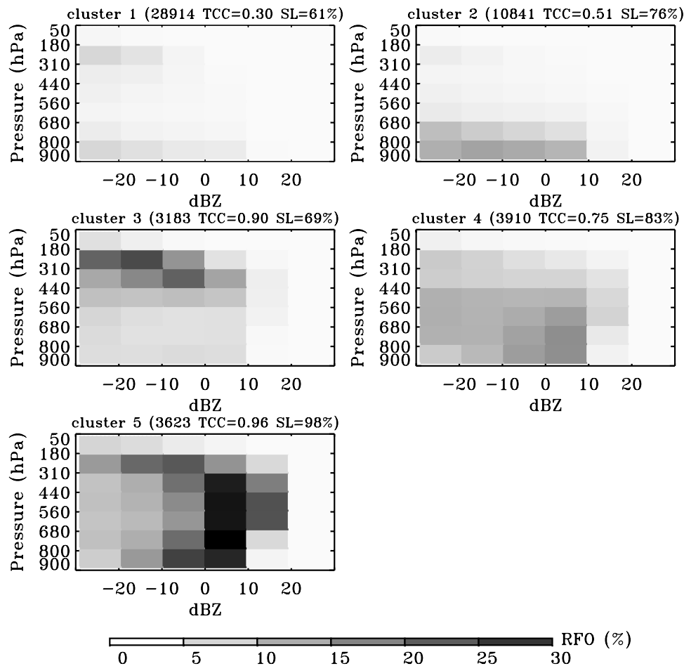
Figure 1. H-dBZ histograms of the centroids of the five clusters. Cluster 1, low cloud and thin cirrus; Cluster 2, subtropical marine stratus; Cluster 3, anvil cirrus cloud; Cluster 4, cumulus congestus; and Cluster 5, deep convection and heavy precipitation. The first number in brackets is the number of elements in each cluster. TCC is the total cloud cover which is the fraction of CloudSat profiles that contain cloud or/and precipitation. SL is, by considering a 200 profile average, the percentage of elements with a single cloud layer, where separate layers are defined by a separation of cloudy range gates by 2 or more non-cloudy range gates.
