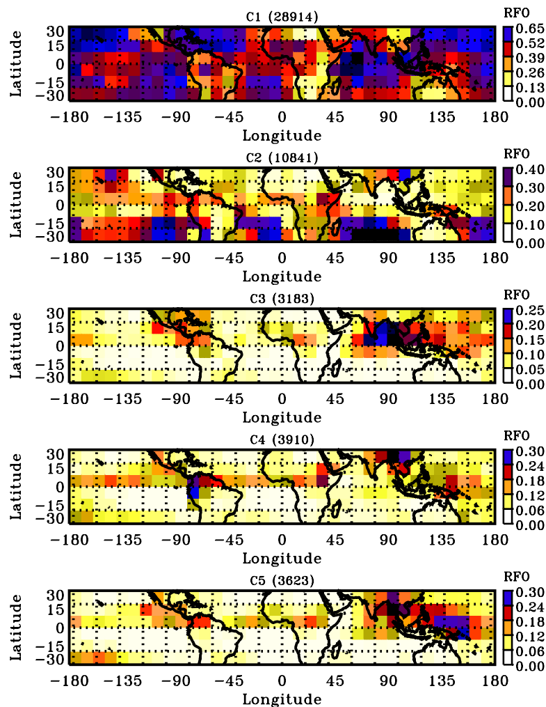
Figure 3. The three-month average occurrence fraction of each cluster. The sum of the frequencies across the clusters in a given 10^\circ -by- 10^\circ box represents the frequency of cloudy elements.
